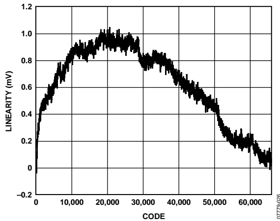
Figure 7. Force Voltage Linearity vs. Code, V_{REF} = 5\text{ V} , No Load
